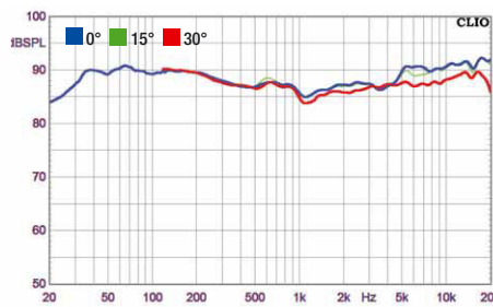
Frequenzgang
